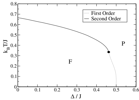
Figure 1. Phase diagram of the Blume–Capel model in the plane k_B T/J - \Delta/J within the mean-field approach, where k_B is the Boltzmann constant, T is the temperature, J > 0 is the coupling constant between each pair of spins and \Delta is the crystal field (also called the anisotropy field), which is regarded constant (without disorder) for each site i . The black circle represents the tricritical point. The ferromagnetic and paramagnetic phases are represented by F and P , respectively. The full line represents the continuous or second-order critical frontier, and the dotted line is for the first-order frontier.
